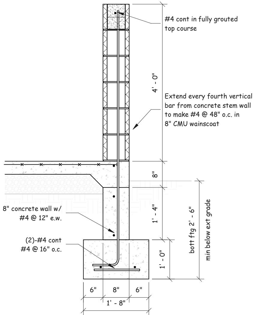
1 Typical Perimeter Stem Wall 1/S5.1 3/4" = 1'-0"
